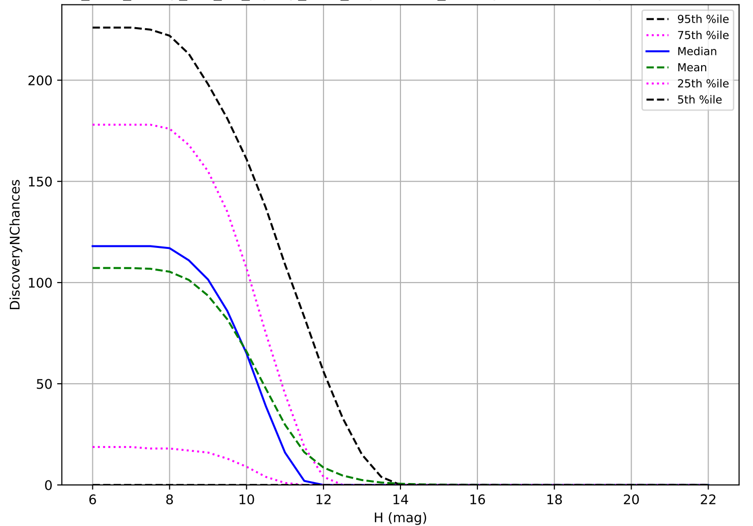
too_elab_heavy_r32_d3_ugrizy_v3.4_10yrs: OCC_r20 3 pairs in 15 nights detection loss
