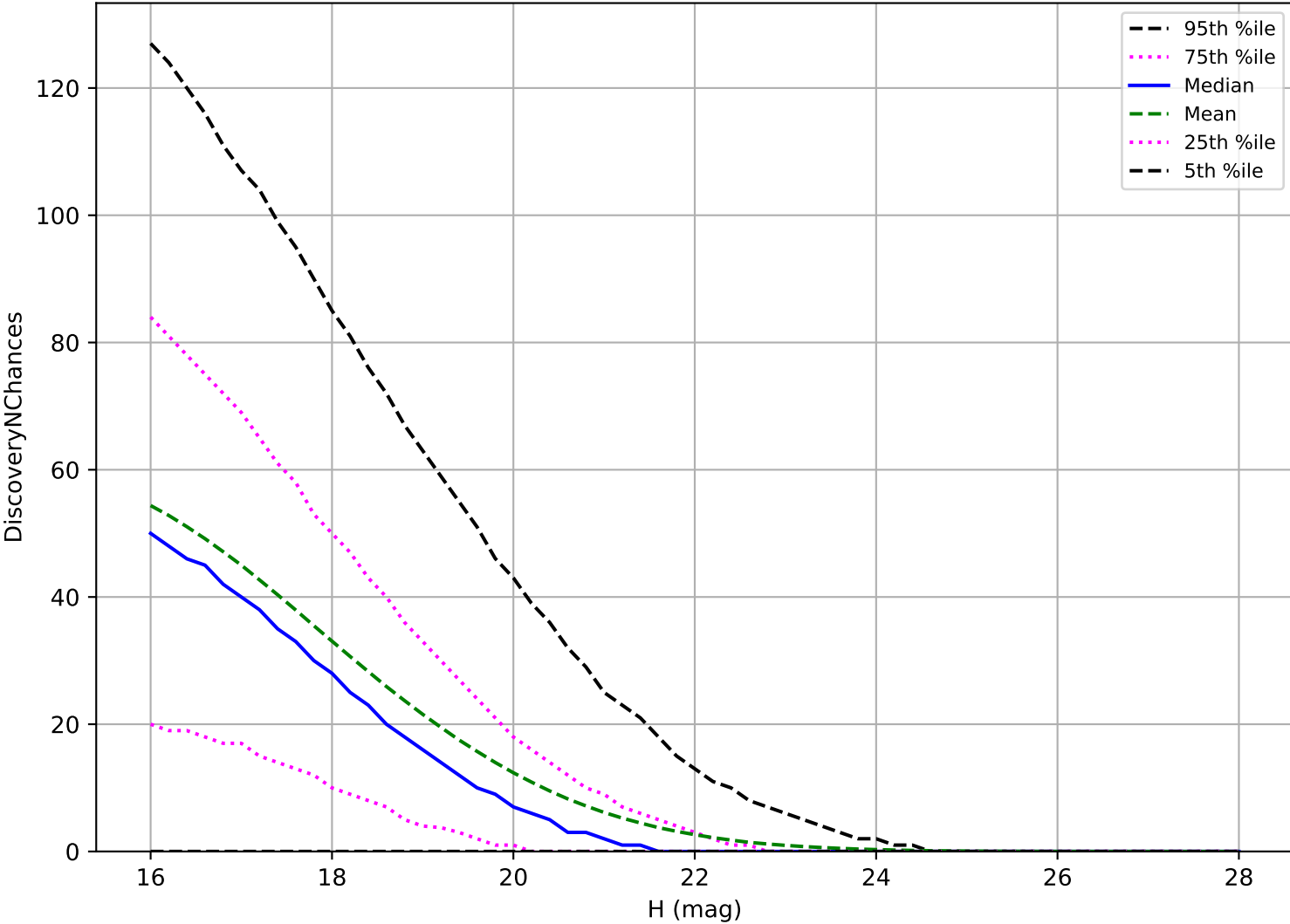
too_elab_heavy_r32_d3_ugrizy_v3.4_10yrs: NEO 3 pairs in 15 nights detection loss
