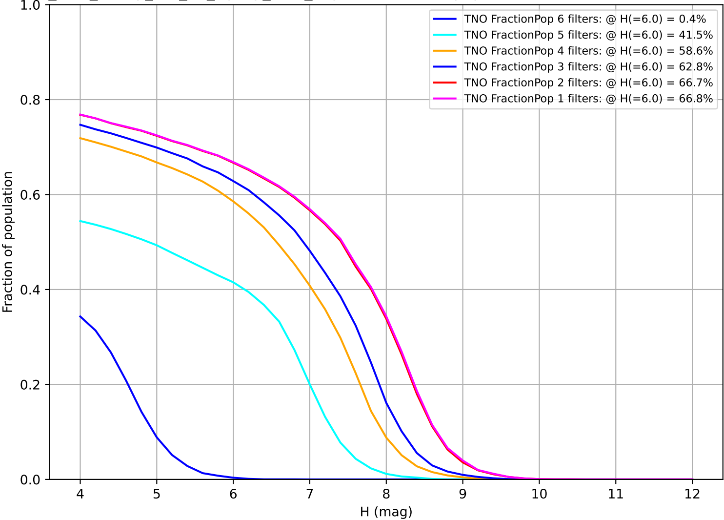
too_elab_heavy_r32_d3_ugrizy_v3.4_10yrs: Fraction of population with colors in X filters TNO
