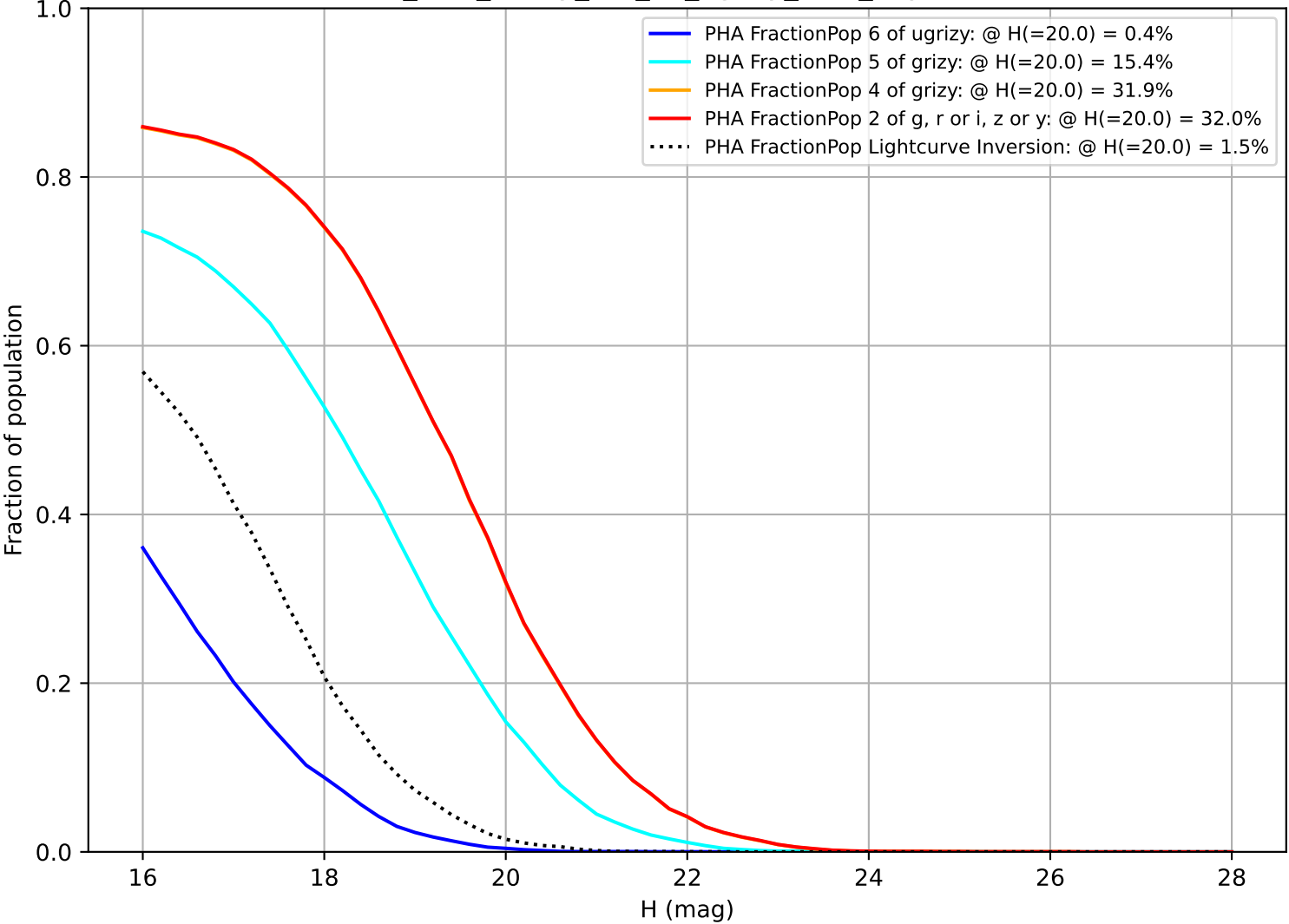
too_elab_heavy_r32_d3_ugrizy_v3.4_10yrs PHA
