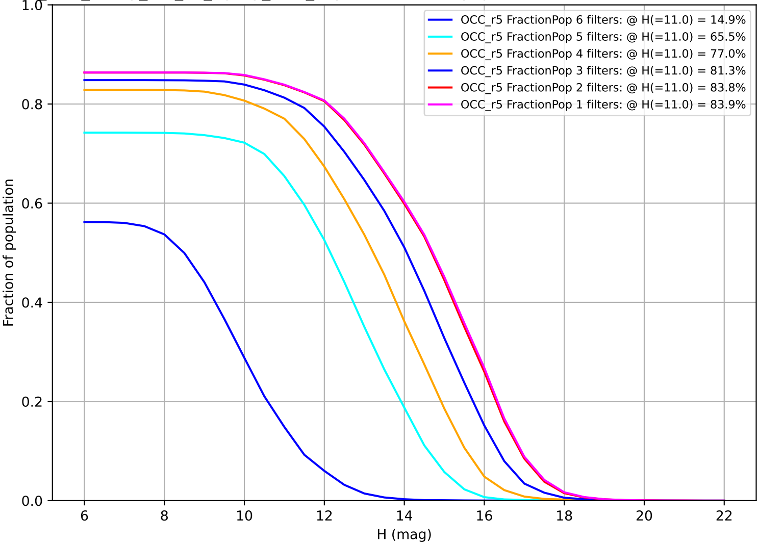
too_elab_heavy_r32_d3_ugrizy_v3.4_10yrs: Fraction of population with colors in X filters OCC_r5
