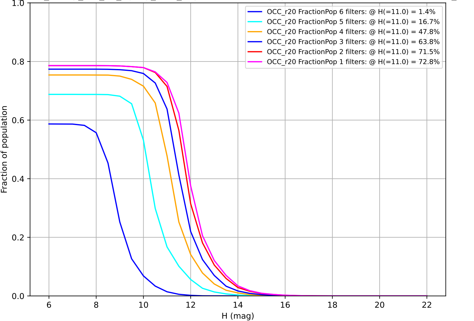
too_elab_heavy_r32_d3_ugrizy_v3.4_10yrs: Fraction of population with colors in X filters OCC_r20
