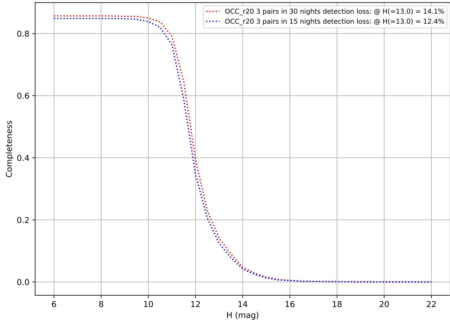
too_elab_heavy_r32_d3_ugrizy_v3.4_10yrs: DifferentialCompleteness
