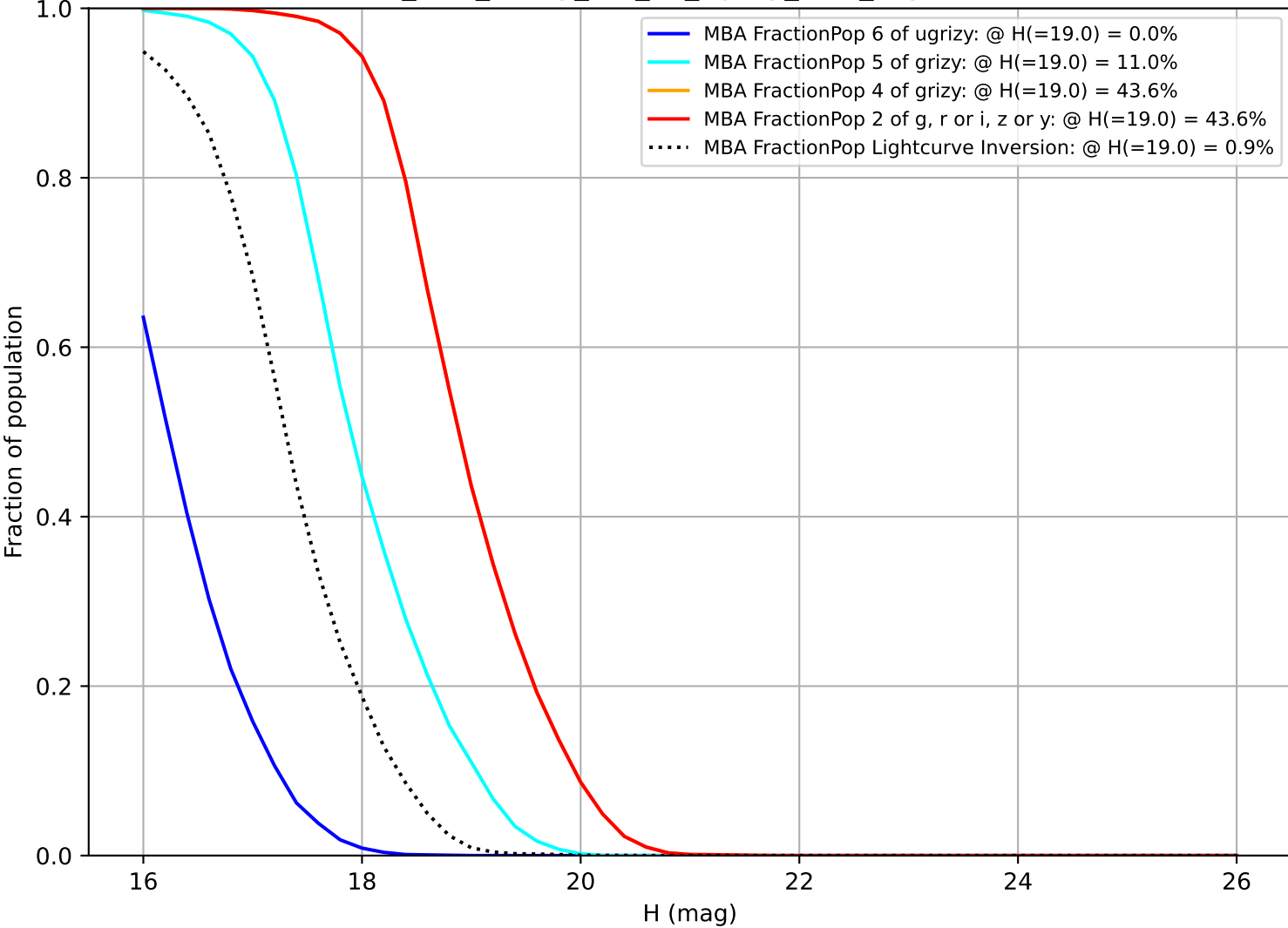
too_elab_heavy_r32_d3_ugrizy_v3.4_10yrs MBA
