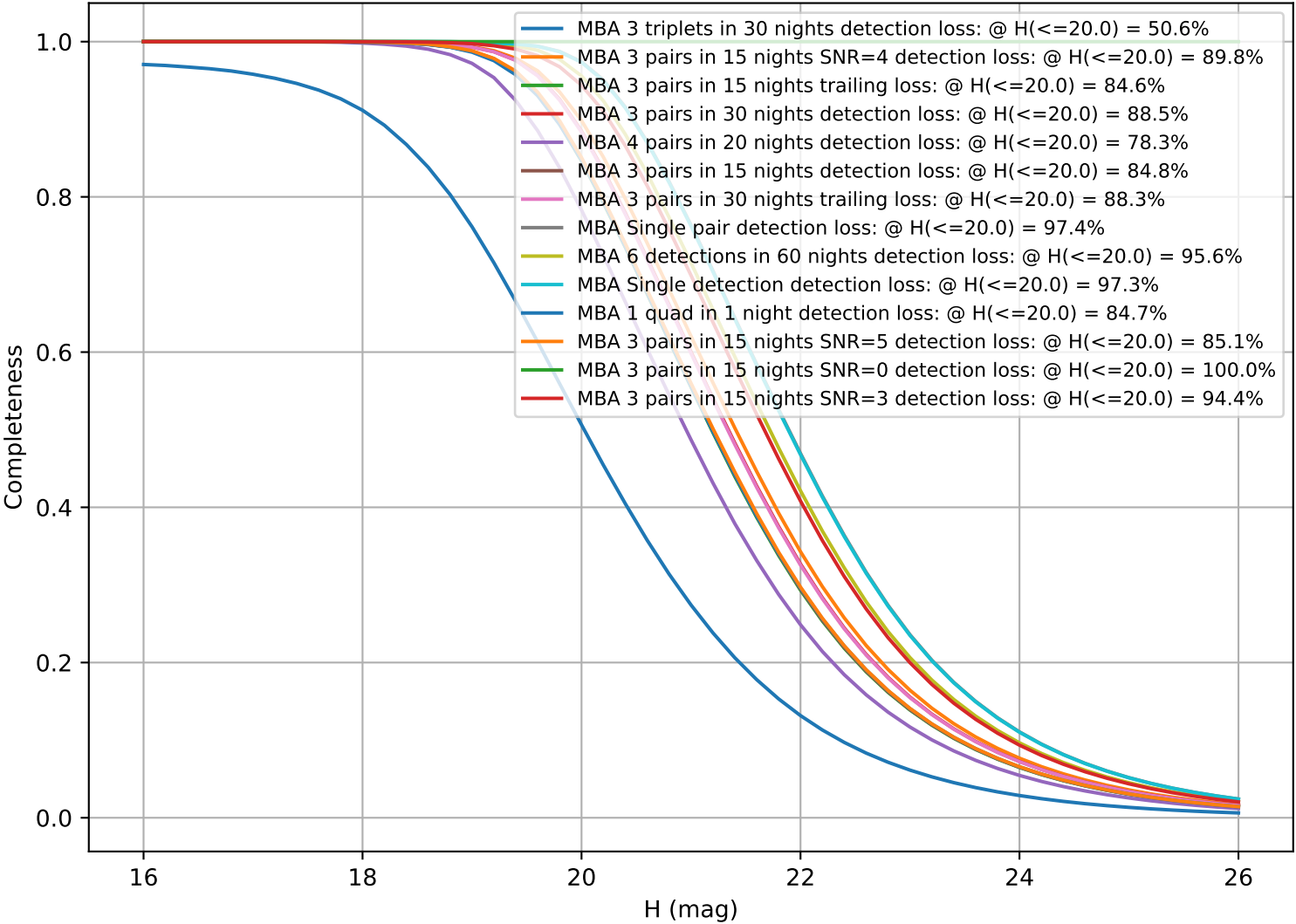
too_elab_heavy_r32_d3_ugrizy_v3.4_10yrs: CumulativeCompleteness
