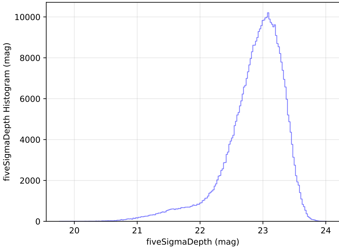
too_elab_heavy_r32_d3_ugrizy_v3.4_10yrs z: fiveSigmaDepth Histogram
