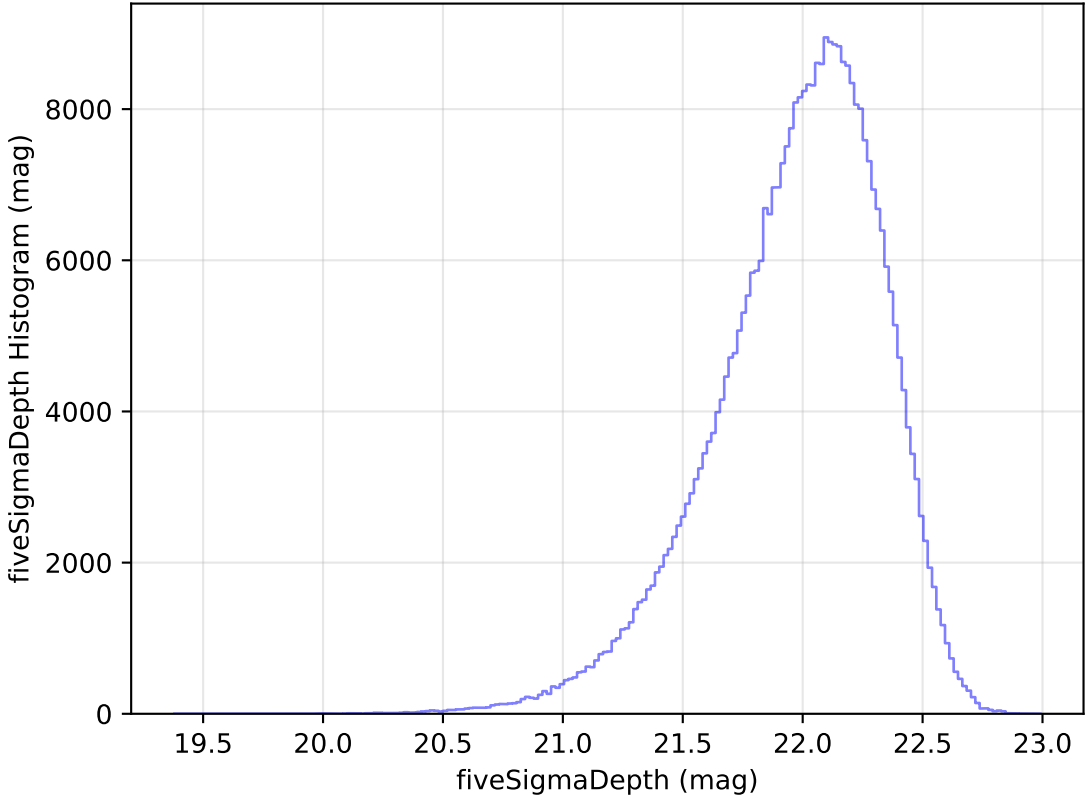
too_elab_heavy_r32_d3_ugrizy_v3.4_10yrs y: fiveSigmaDepth Histogram
