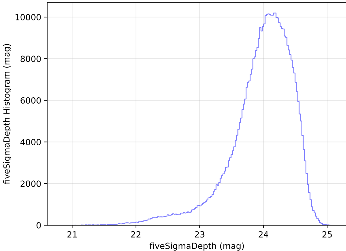
too_elab_heavy_r32_d3_ugrizy_v3.4_10yrs r: fiveSigmaDepth Histogram
