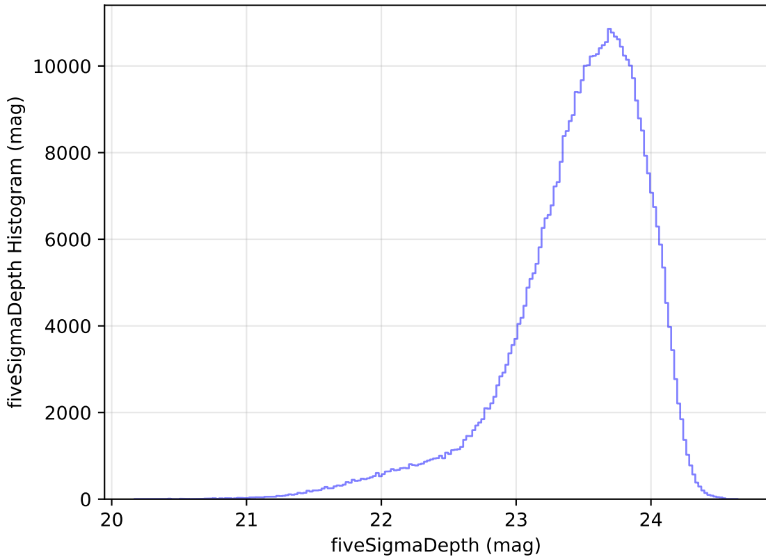
too_elab_heavy_r32_d3_ugrizy_v3.4_10yrs i: fiveSigmaDepth Histogram
