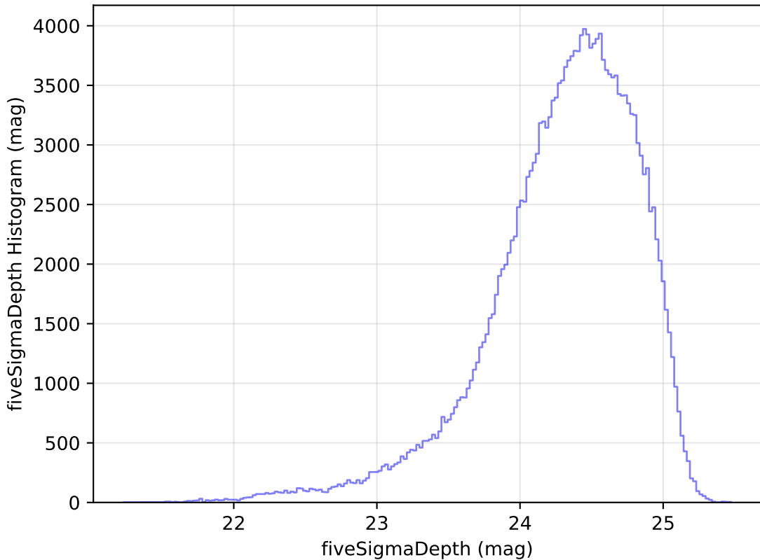
too_elab_heavy_r32_d3_ugrizy_v3.4_10yrs g: fiveSigmaDepth Histogram
