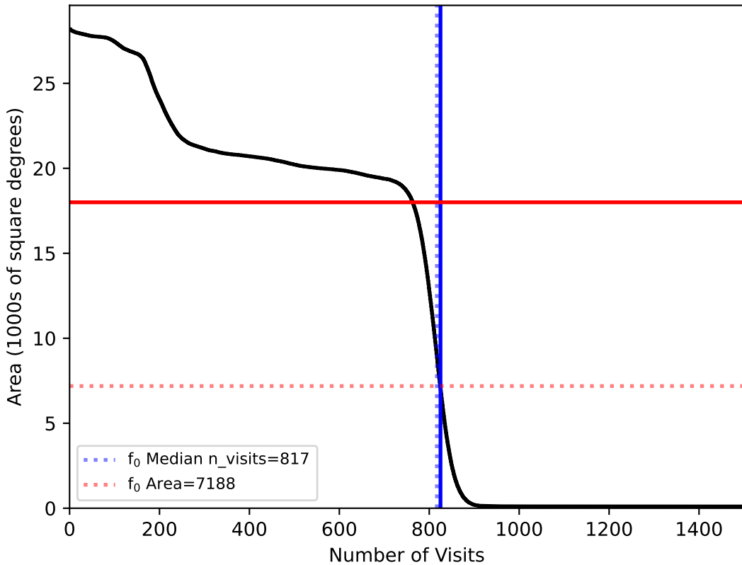
too_elab_heavy_r32_d3_ugrizy_v3.4_10yrs : f0
