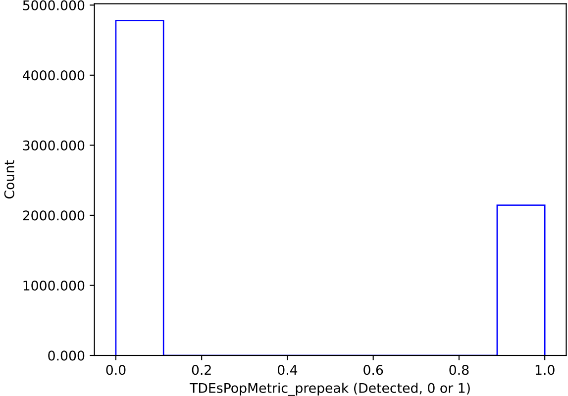
too_elab_heavy_r32_d3_ugrizy_v3.4_10yrs : TDEsPopMetric_prepeak
