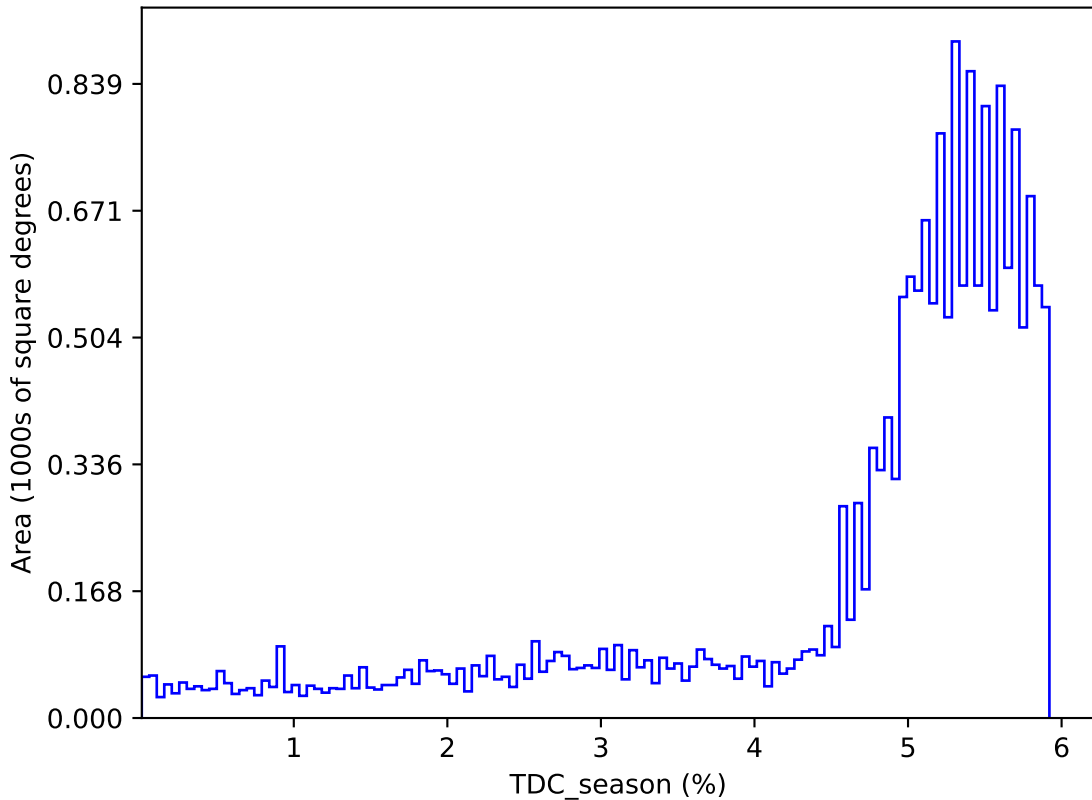
too_elab_heavy_r32_d3_ugrizy_v3.4_10yrs : TDC_season
