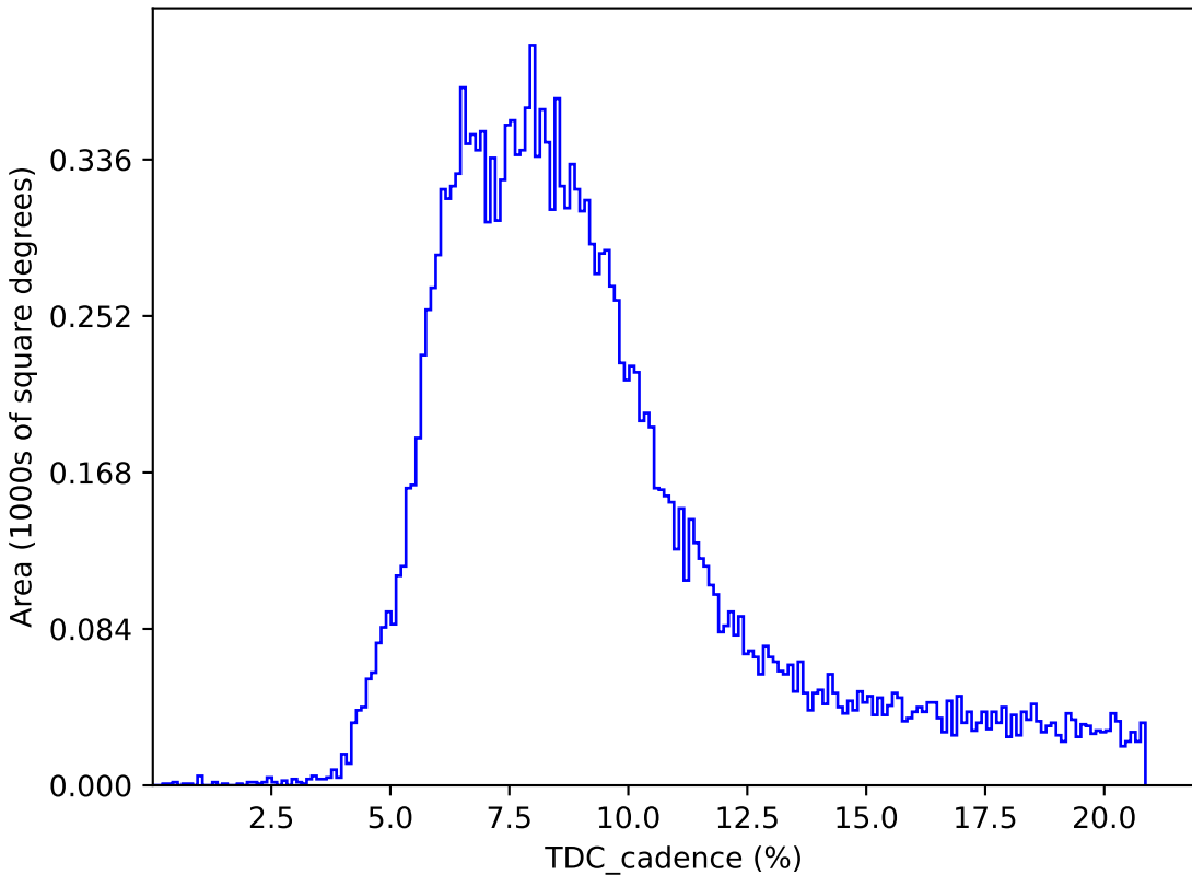
too_elab_heavy_r32_d3_ugrizy_v3.4_10yrs : TDC_cadence
