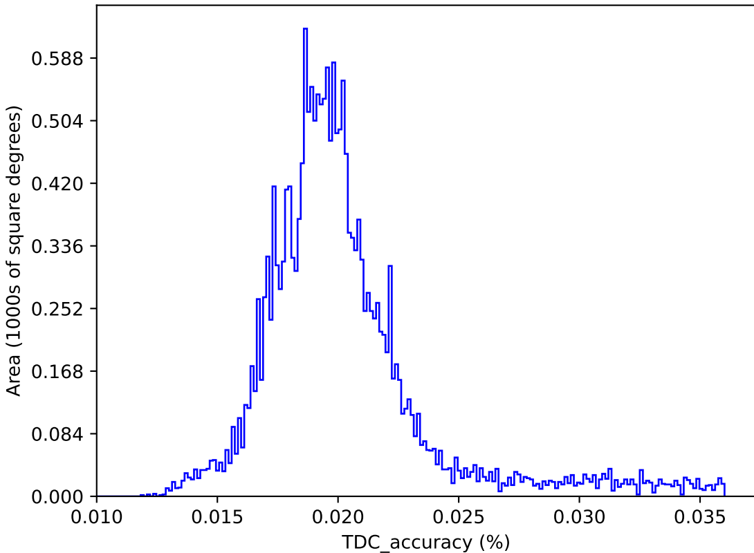
too_elab_heavy_r32_d3_ugrizy_v3.4_10yrs : TDC_accuracy
