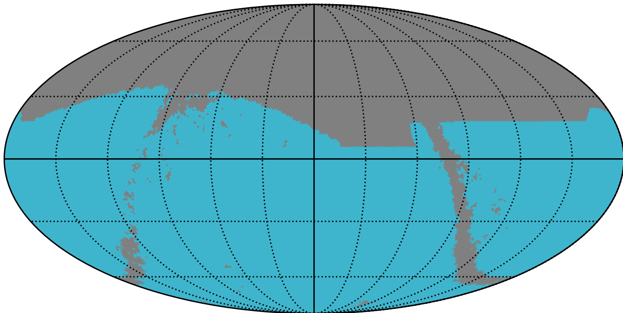
too_elab_heavy_r32_d3_ugrizy_v3.4_10yrs : SNSLMetric
