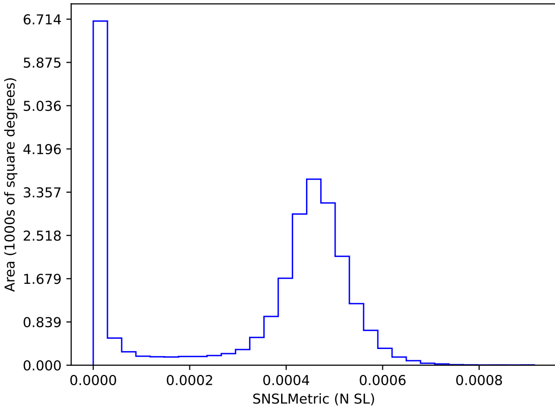
too_elab_heavy_r32_d3_ugrizy_v3.4_10yrs : SNSLMetric
