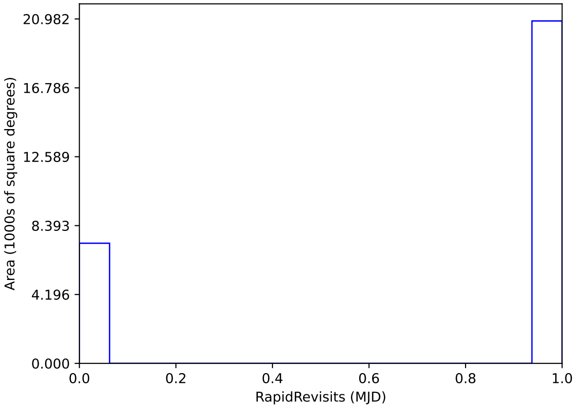
too_elab_heavy_r32_d3_ugrizy_v3.4_10yrs : RapidRevisits
