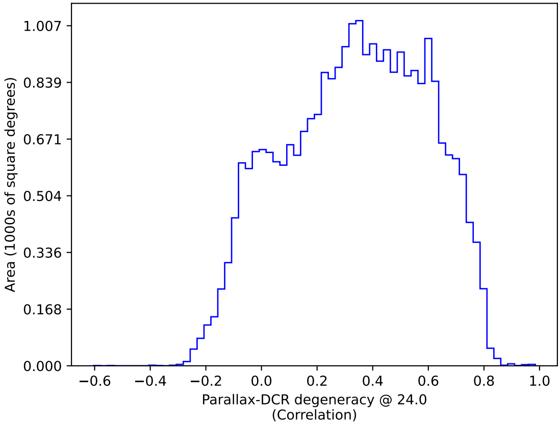
too_elab_heavy_r32_d3_ugrizy_v3.4_10yrs : Parallax-DCR degeneracy @ 24.0
