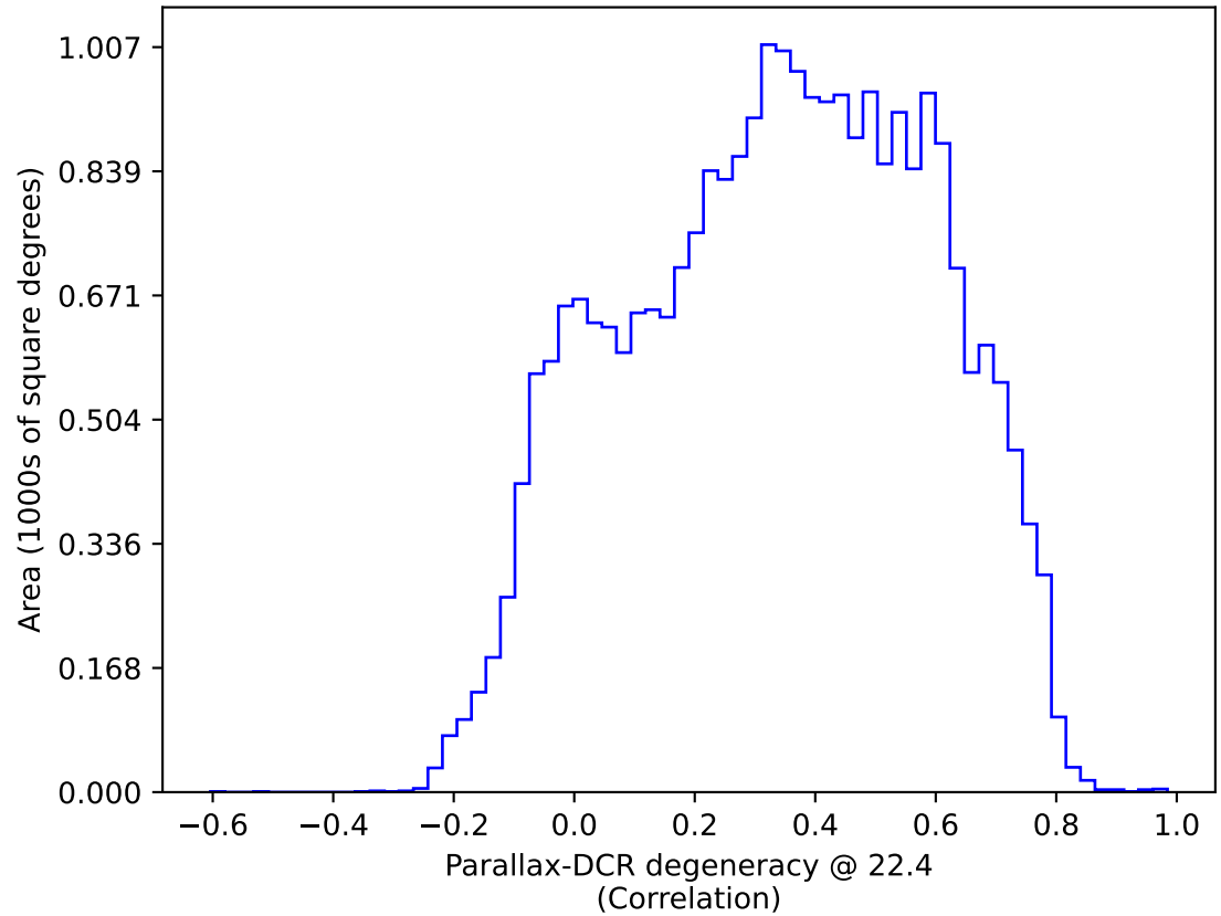
too_elab_heavy_r32_d3_ugrizy_v3.4_10yrs : Parallax-DCR degeneracy @ 22.4
