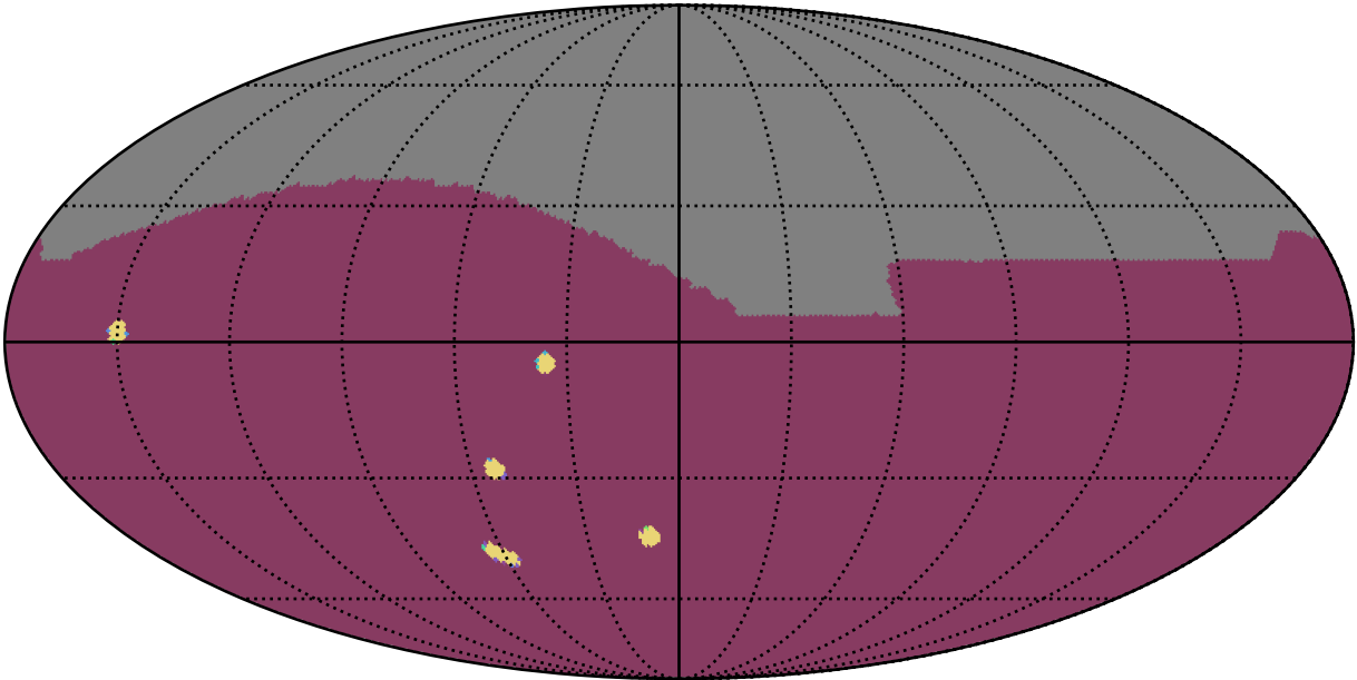
too_elab_heavy_r32_d3_ugrizy_v3.4_10yrs : NumberOfQuickRevisits
