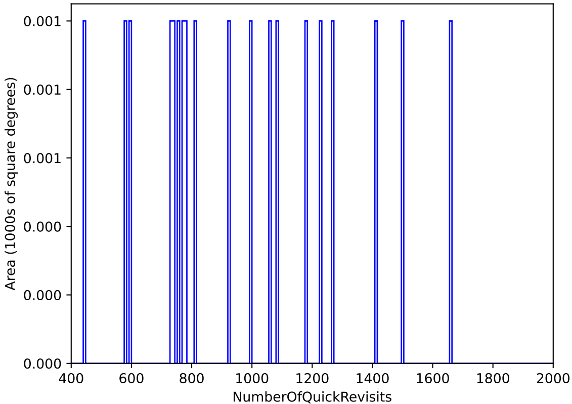
too_elab_heavy_r32_d3_ugrizy_v3.4_10yrs : NumberOfQuickRevisits
