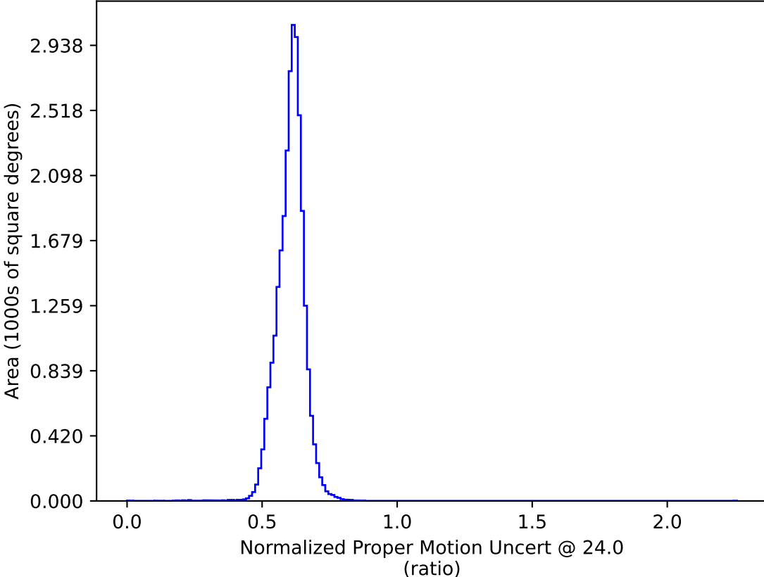
too_elab_heavy_r32_d3_ugrizy_v3.4_10yrs : Normalized Proper Motion Uncert @ 24.0
