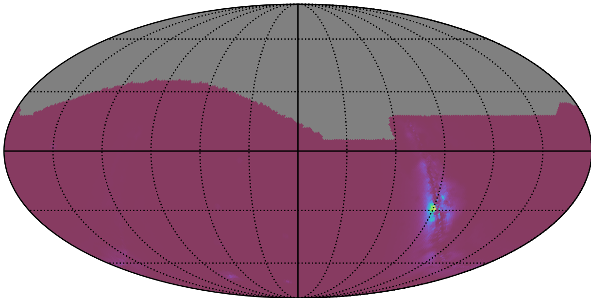
too_elab_heavy_r32_d3_ugrizy_v3.4_10yrs : NlcPoints
