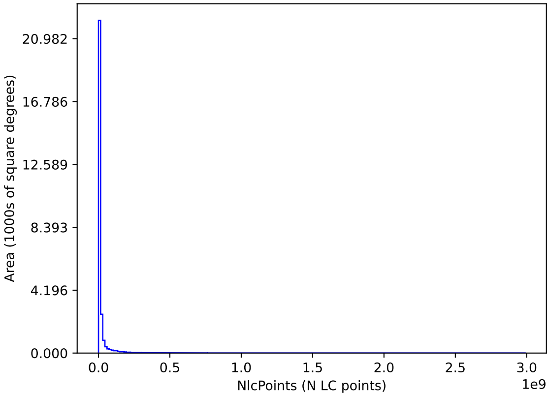
too_elab_heavy_r32_d3_ugrizy_v3.4_10yrs : NlcPoints
