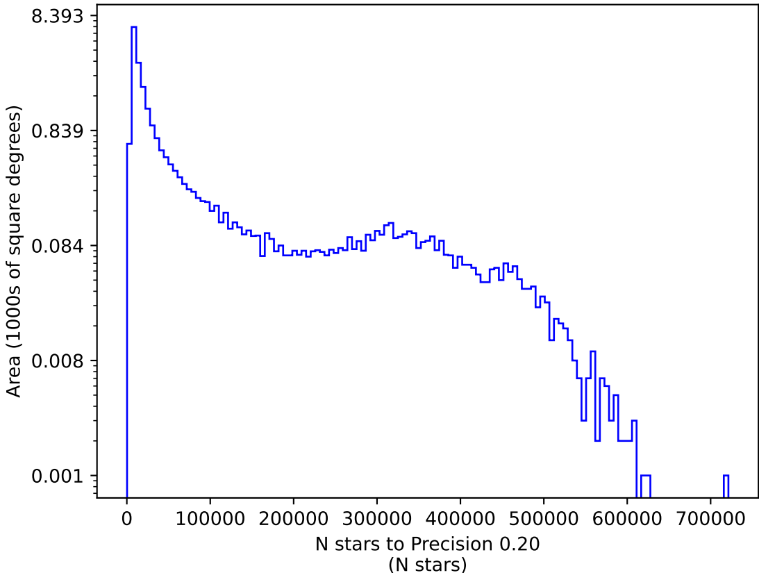
too_elab_heavy_r32_d3_ugrizy_v3.4_10yrs y: N stars to Precision 0.20
