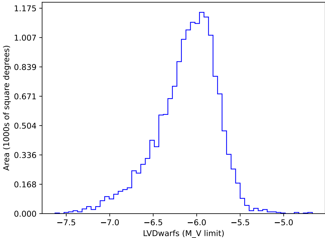
too_elab_heavy_r32_d3_ugrizy_v3.4_10yrs gi: LVDwarfs
