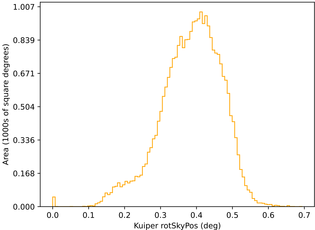
too_elab_heavy_r32_d3_ugrizy_v3.4_10yrs r: Kuiper rotSkyPos
