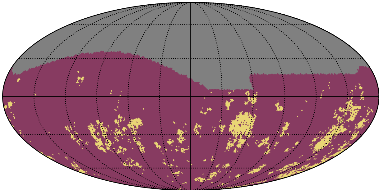
too_elab_heavy_r32_d3_ugrizy_v3.4_10yrs g band: Gaps_7hr
