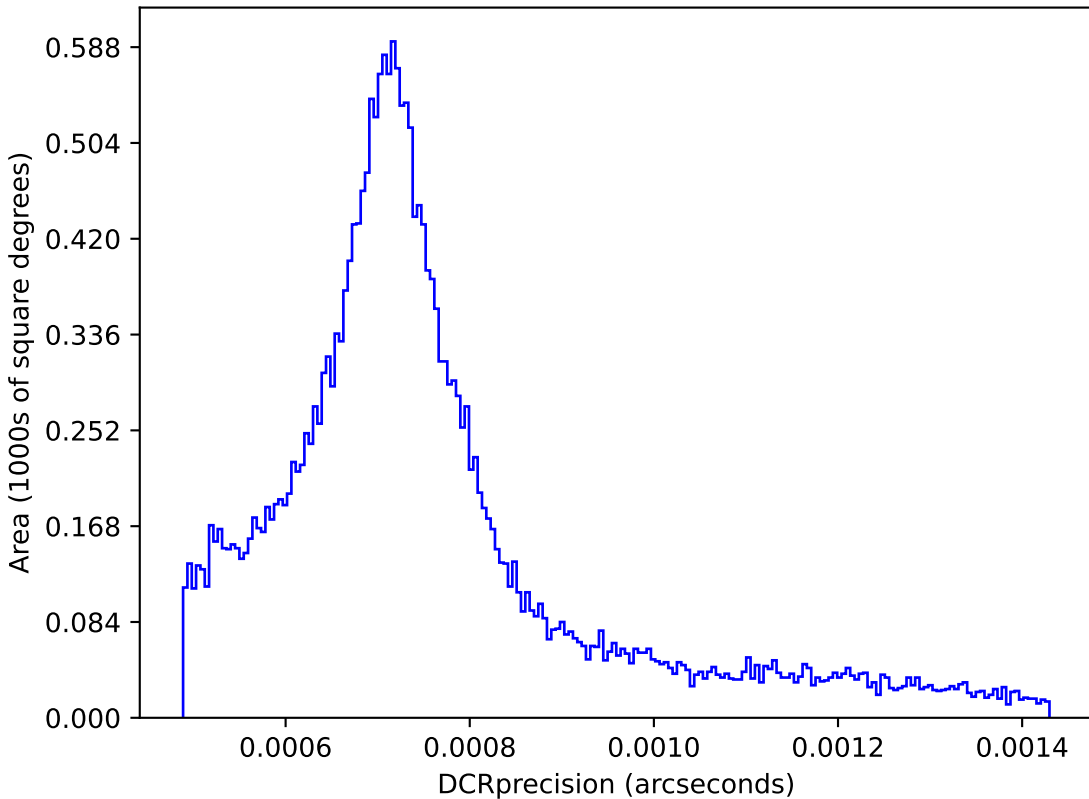
too_elab_heavy_r32_d3_ugrizy_v3.4_10yrs : DCRprecision
