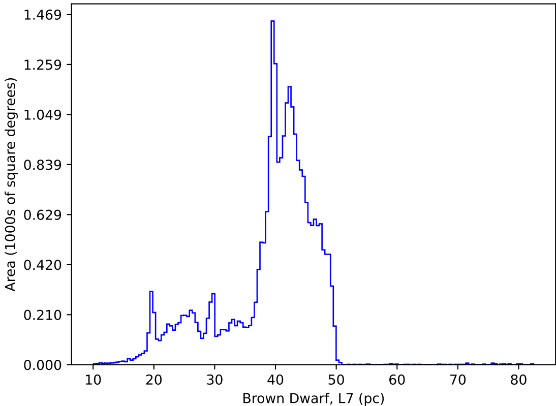
too_elab_heavy_r32_d3_ugrizy_v3.4_10yrs : Brown Dwarf, L7
