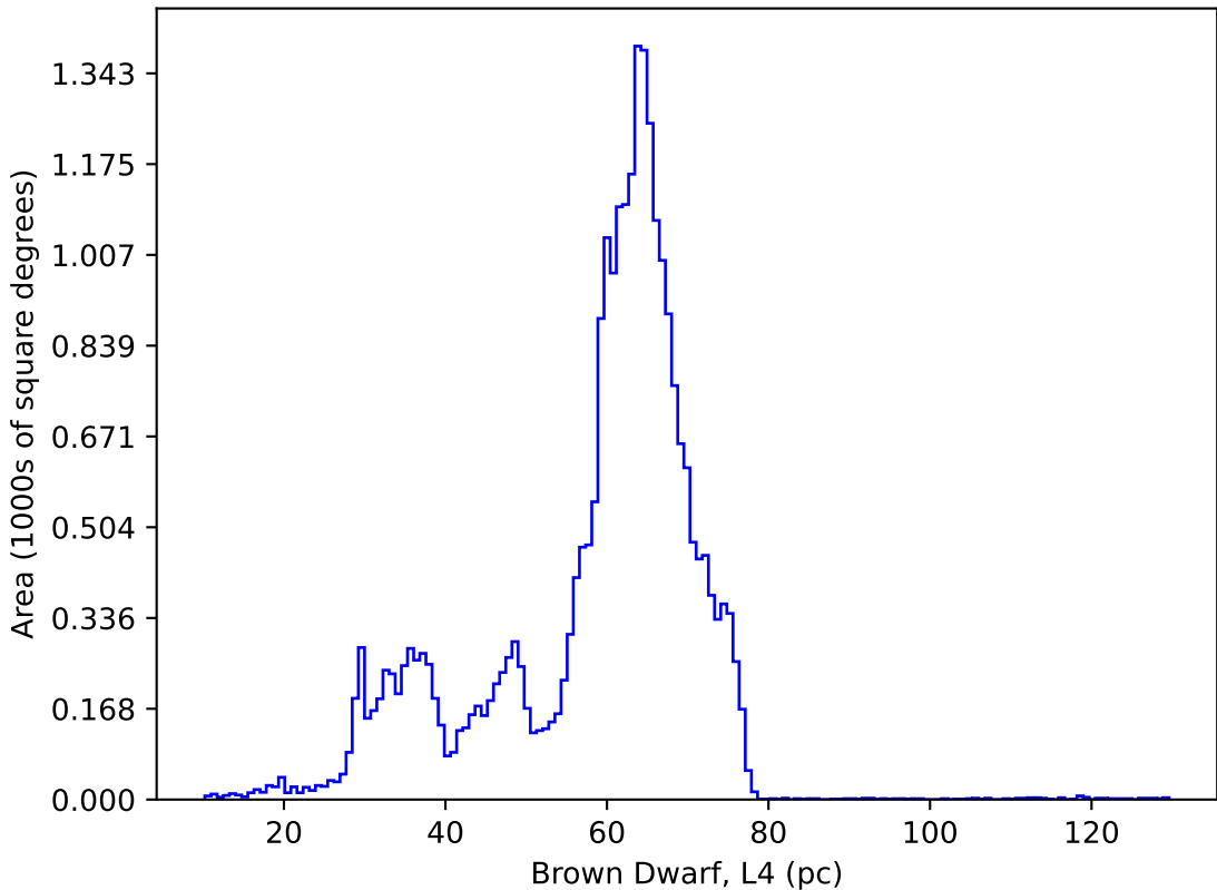
too_elab_heavy_r32_d3_ugrizy_v3.4_10yrs : Brown Dwarf, L4
