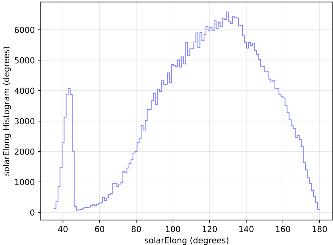
too_elab_heavy_r32_d3_ugrizy_v3.4_10yrs WFD z band: solarElong Histogram
