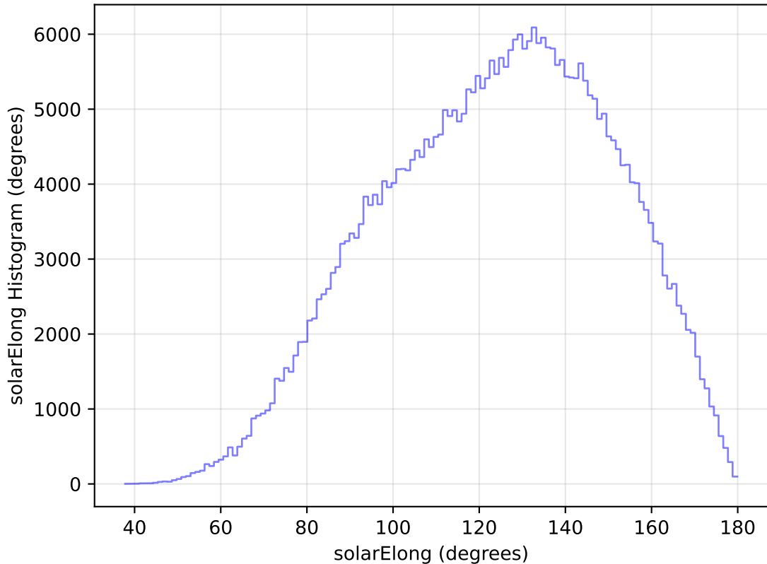
too_elab_heavy_r32_d3_uigrizy_v3.4_10yrs WFD y band: solarElong Histogram
