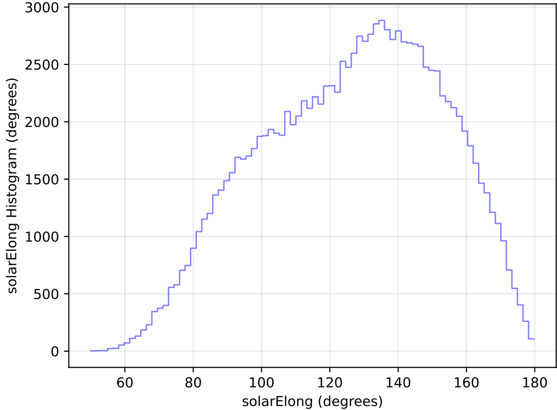
too_elab_heavy_r32_d3_ugrizy_v3.4_10yrs WFD u band: solarElong Histogram
