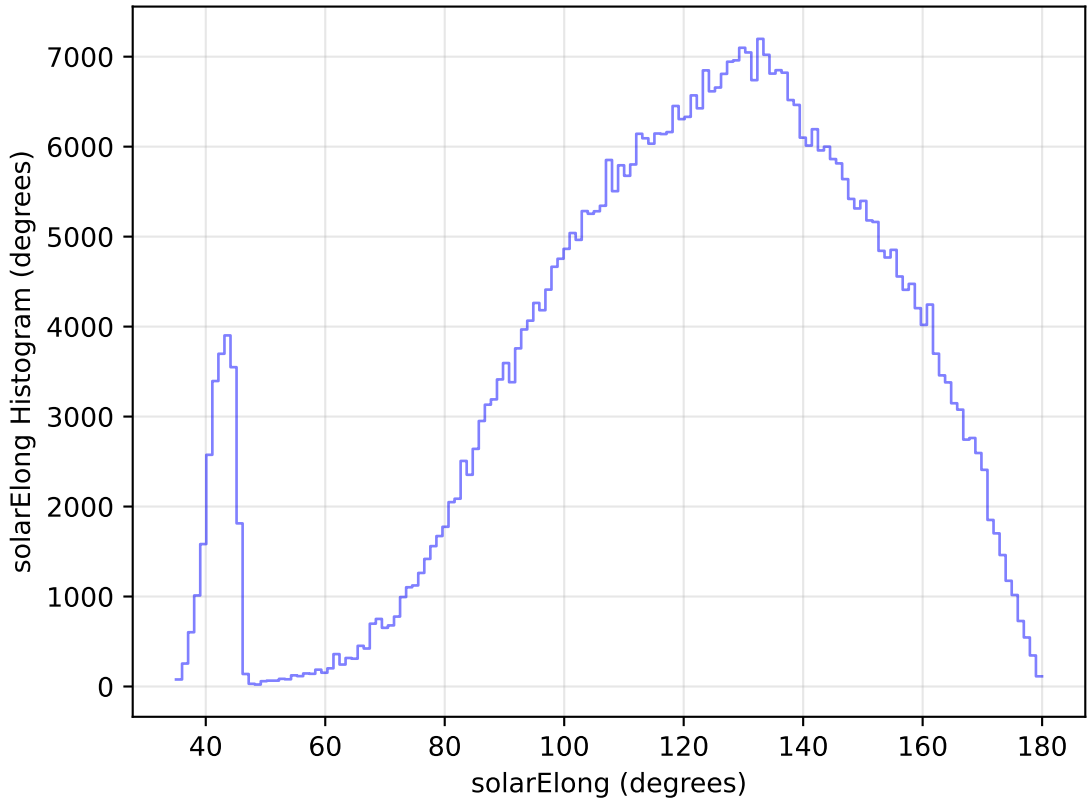
too_elab_heavy_r32_d3_ugrizy_v3.4_10yrs WFD i band: solarElong Histogram
