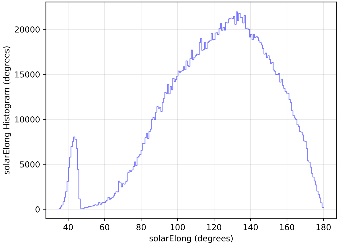
too_elab_heavy_r32_d3_ugrizy_v3.4_10yrs WFD all bands: solarElong Histogram
