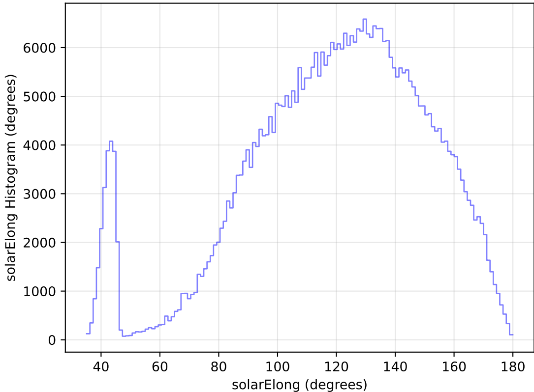
too_elab_heavy_r32_d3_ugrizy_v3.4_10yrs All sky z band: solarElong Histogram
