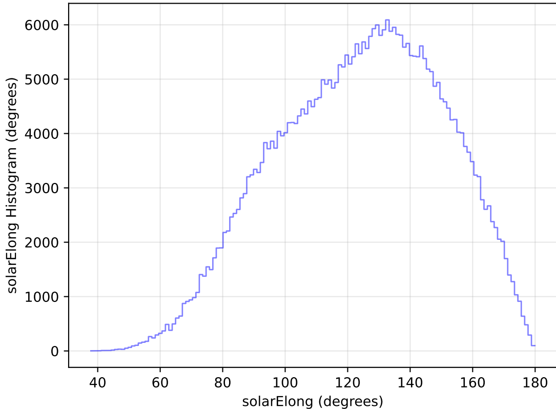
too_elab_heavy_r32_d3_ugrizy_v3.4_10yrs All sky y band: solarElong Histogram
