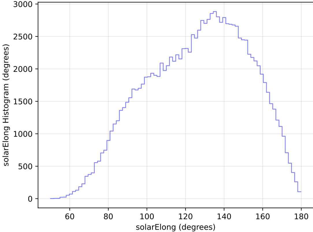
too_elab_heavy_r32_d3_ugrizy_v3.4_10yrs All sky u band: solarElong Histogram
