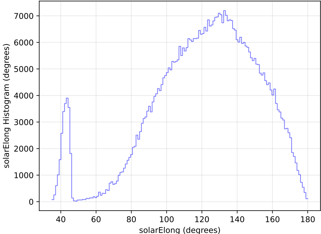
too_elab_heavy_r32_d3_ugrizy_v3.4_10yrs All sky i band: solarElong Histogram
