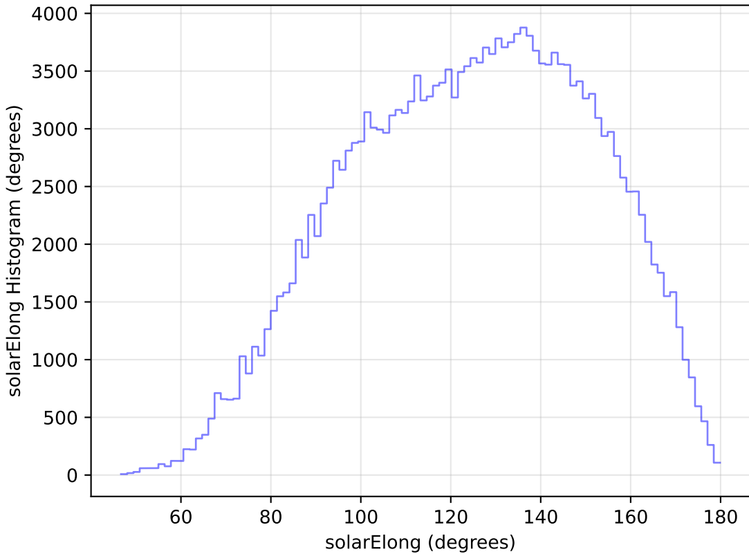
too_elab_heavy_r32_d3_ugrizy_v3.4_10yrs All sky g band: solarElong Histogram
