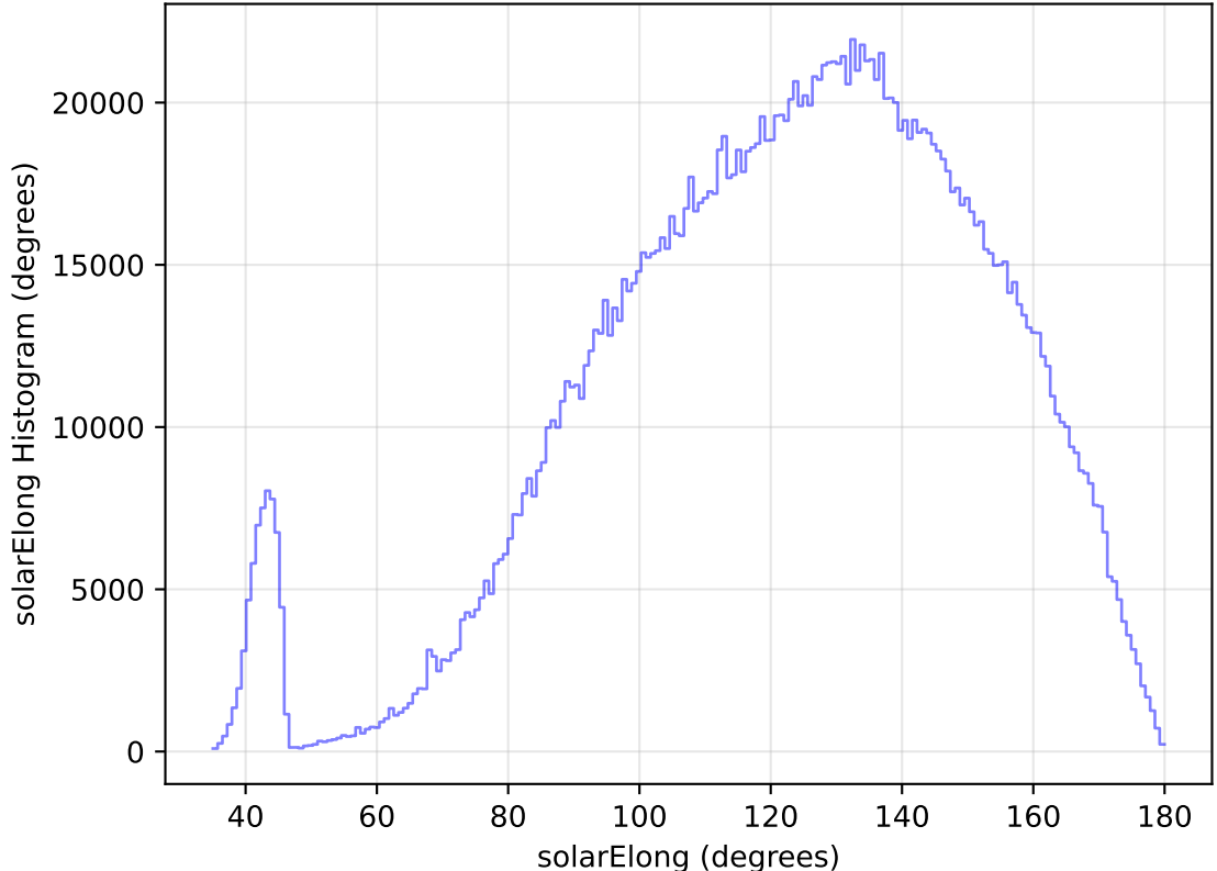
too_elab_heavy_r32_d3_ugrizy_v3.4_10yrs All sky all bands: solarElong Histogram
