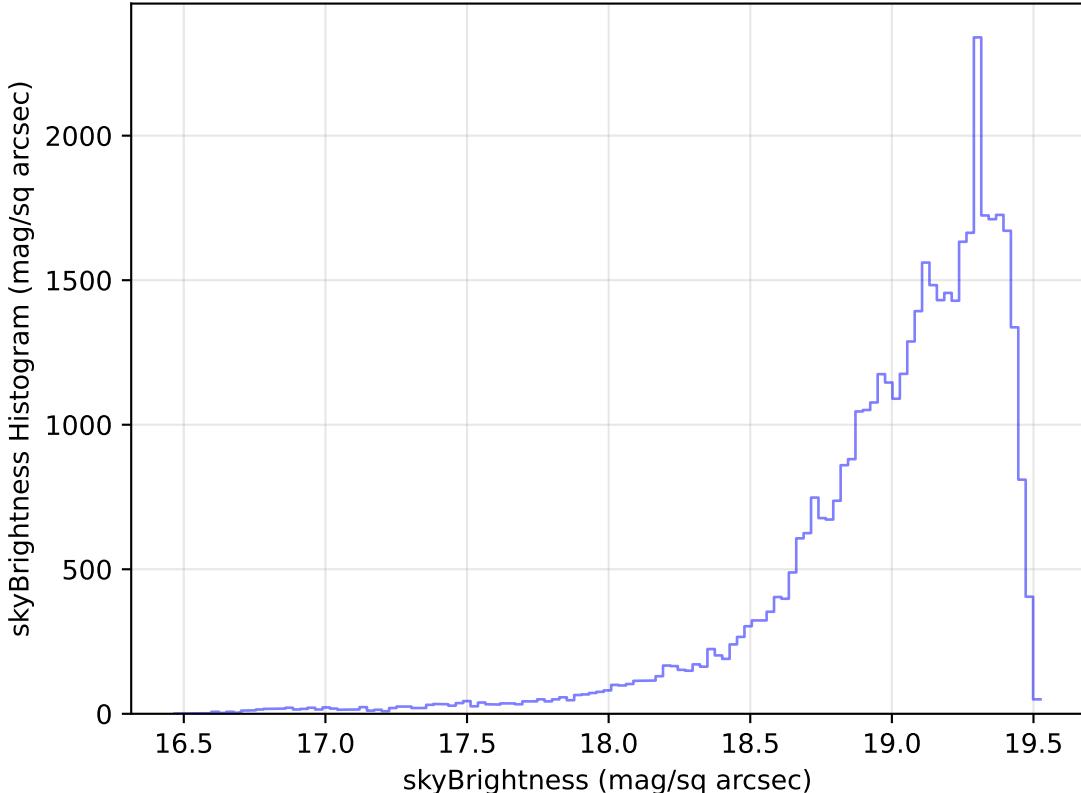
too_elab_heavy_r32_d3_ugrizy_v3.4_10yrs Yr 1 z band: skyBrightness Histogram
