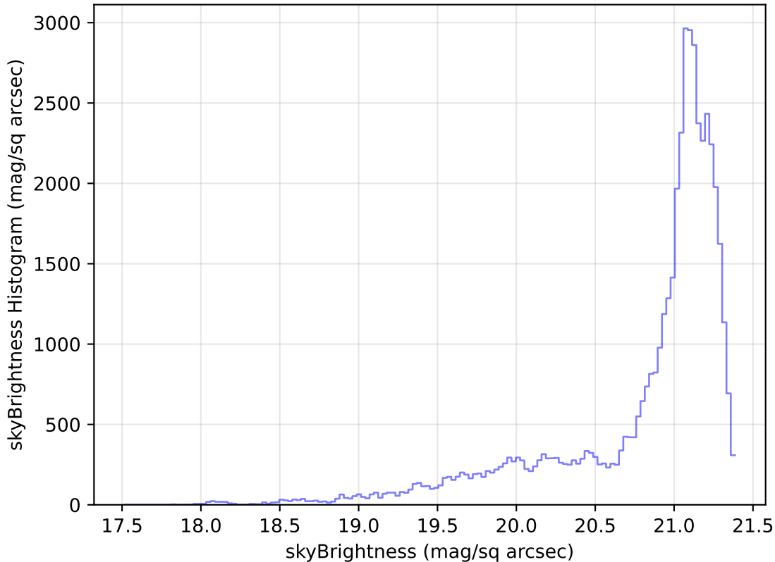
too_elab_heavy_r32_d3_ugrizy_v3.4_10yrs Yr 1 r band: skyBrightness Histogram
