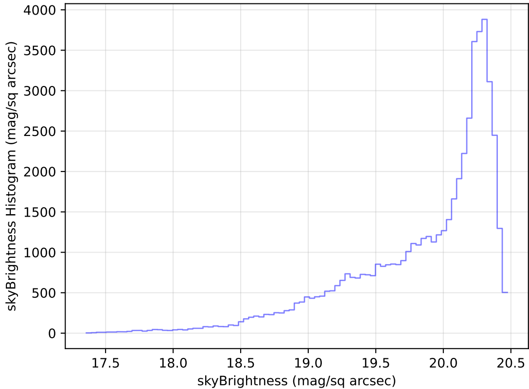
too_elab_heavy_r32_d3_ugrizy_v3.4_10yrs Yr 1 i band: skyBrightness Histogram
